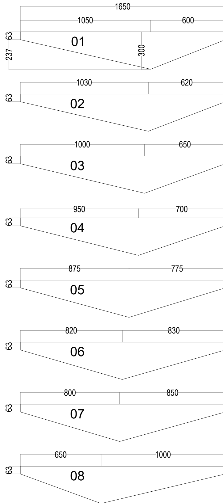
CEILING WOODEN RAFTER ELEVATION
