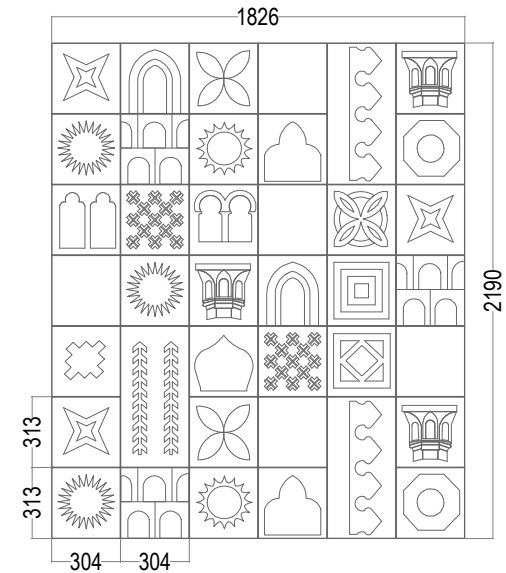
TYPICAL PATTERN FOR CNC CUTTING
