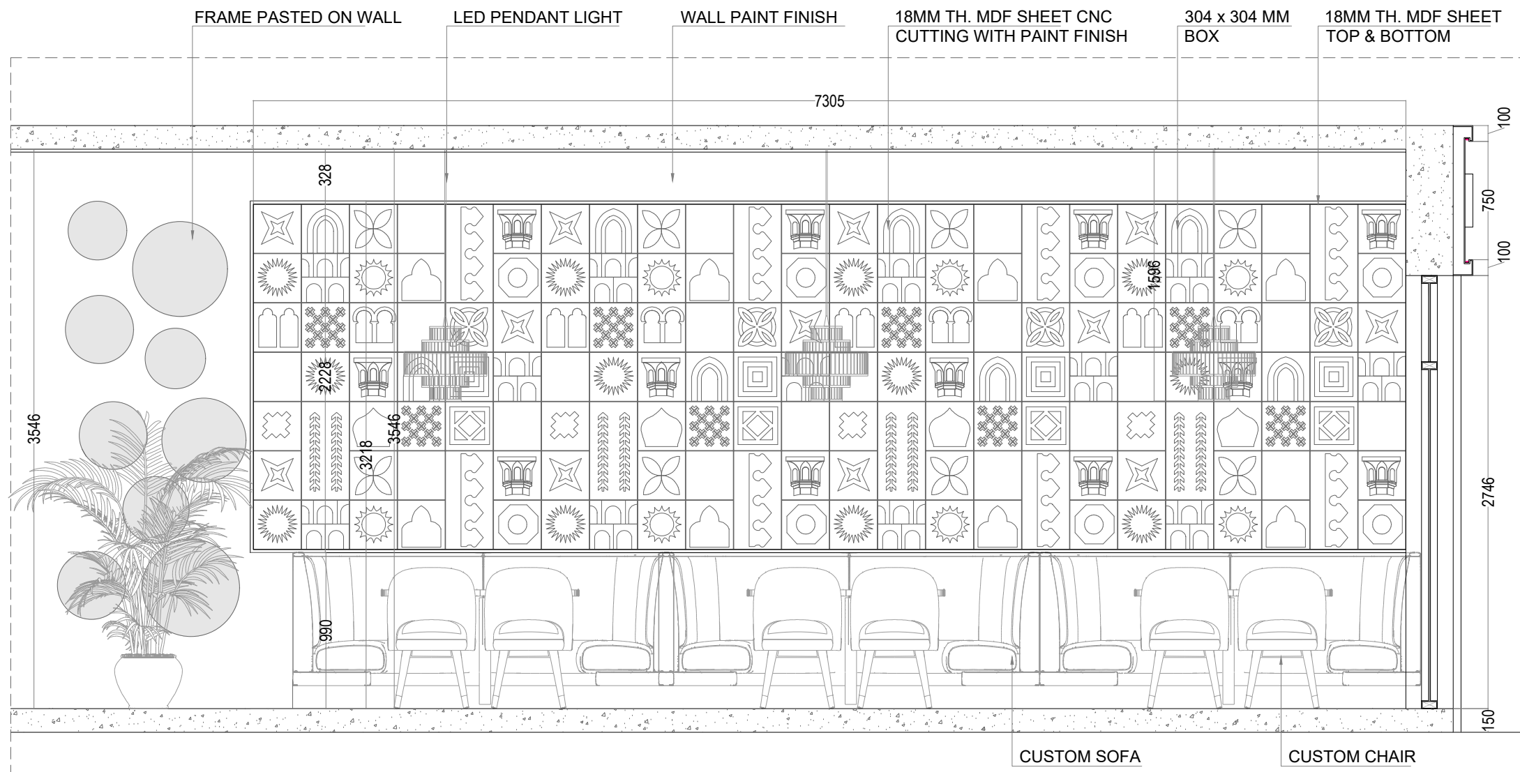
CNC CUTTING FEATURE WALL ELEVATION
