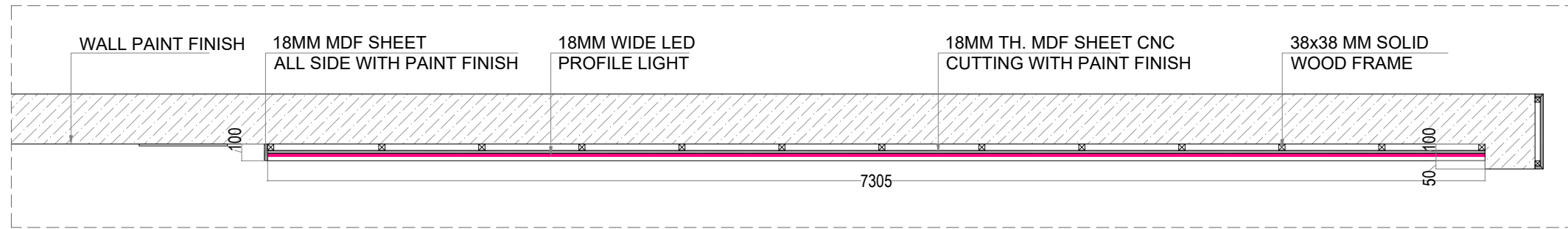
CNC CUTTING FEATURE WALL PLAN
