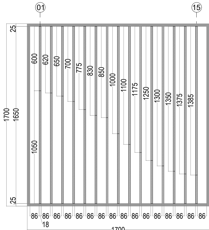
CEILING WOODEN PANEL PLAN
